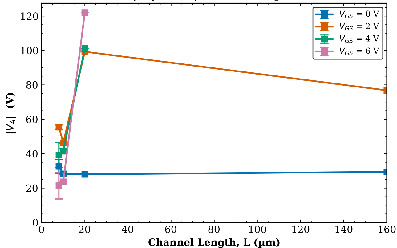
All Chips - Combined |V_A| vs L | W = 1000\text{ }\mu\text{m}
